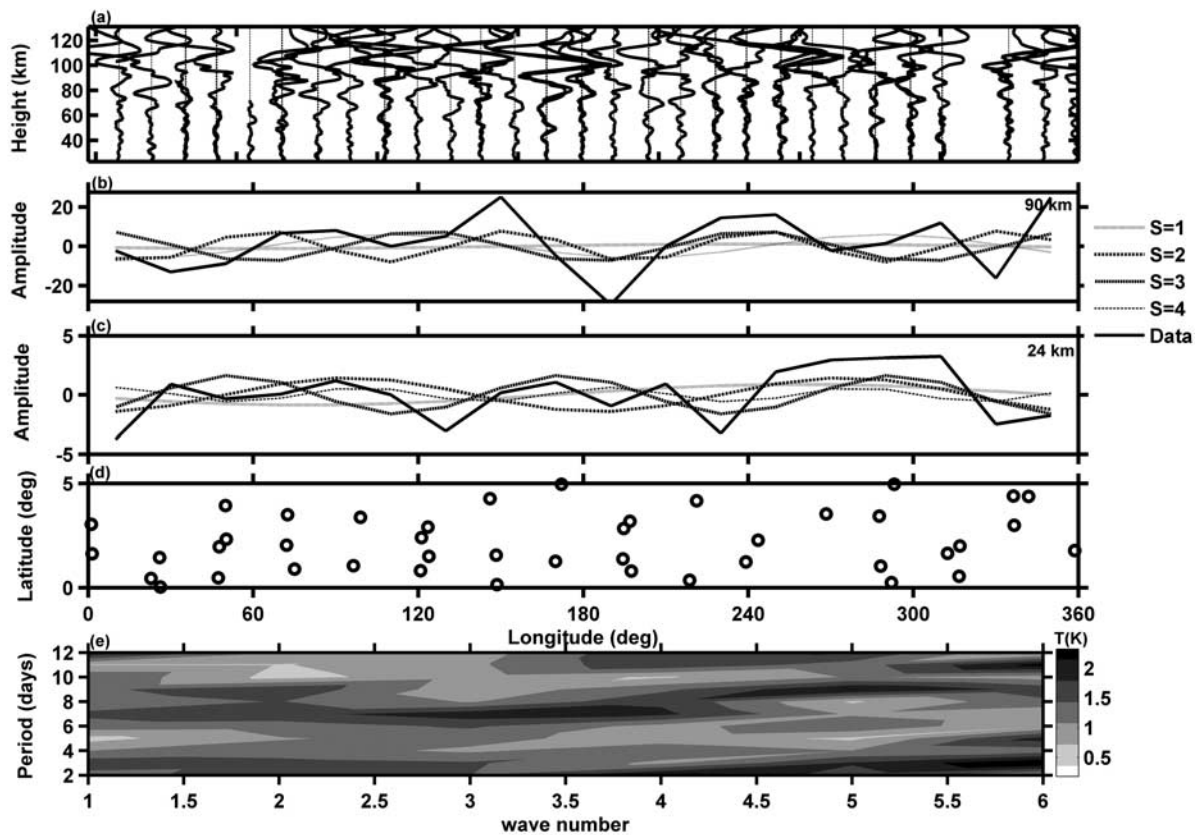
Figure 4. (a) Profiles of temperature fluctuation ( T' ) over 10°N–10°S latitude, longitudinal variations of T' (thick lines), and the fitted T' for wave numbers 1–4 (dotted lines) at an altitude of (b) 90 and (c) 24 km observed on 6 July 2004. Each T' profile (curve) in Figure 4a is plotted at its corresponding longitude (dotted line), where 1 K is equivalent to 3° in longitude. (d) Locations of SABER events on 6 July 2004. (e) Space-time spectral analysis of temperature observations from SABER carried out at 90 km altitude during July–August 2004.
