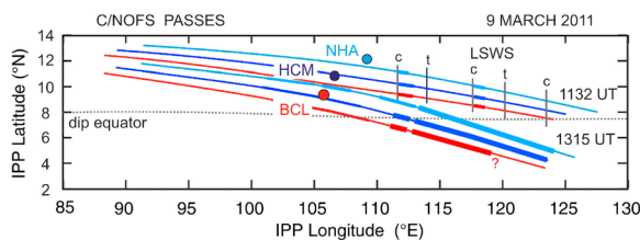
Figure 2. Tracks of the ionospheric penetration points (IPPs) for BCL, HCM, and NHA, for the C/NOFS passes at 1132 and 1315 UT, 9 March 2011.
