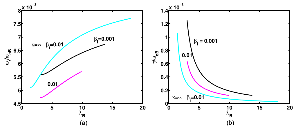
FIG. 8. KAW resonant instability driven by velocity shear: variation of (a) normalized real frequency, \omega_r/\omega_{cB} , and (b) normalized growth rate, \gamma/\omega_{cB} vs \lambda_B = \frac{k_{||}^2 \alpha_B^2}{2\omega_{cB}^2} for S = 0.5 , N_B/N_e = 0.5 , k_{||}/k_{\perp} = 0.01 , \kappa = 3, \infty and various values of \beta_i as listed on the curves.
