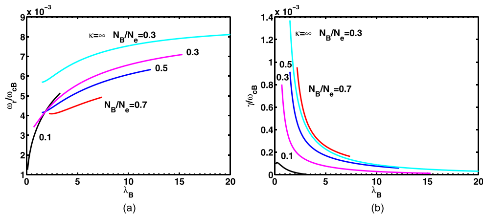
FIG. 5. KAW resonant instability driven by velocity shear: variation of (a) normalized real frequency, \omega_r/\omega_{cB} , and (b) normalized growth rate, \gamma/\omega_{cB} vs \lambda_B = \frac{k_{\perp}^2 \alpha_B^2}{2\omega_{cB}^2} for S = 0.3 , \kappa = (3, \infty) , \beta_i = 0.001 , k_{\parallel}/k_{\perp} = 0.01 and various values of N_B/N_e as listed on the curves.
