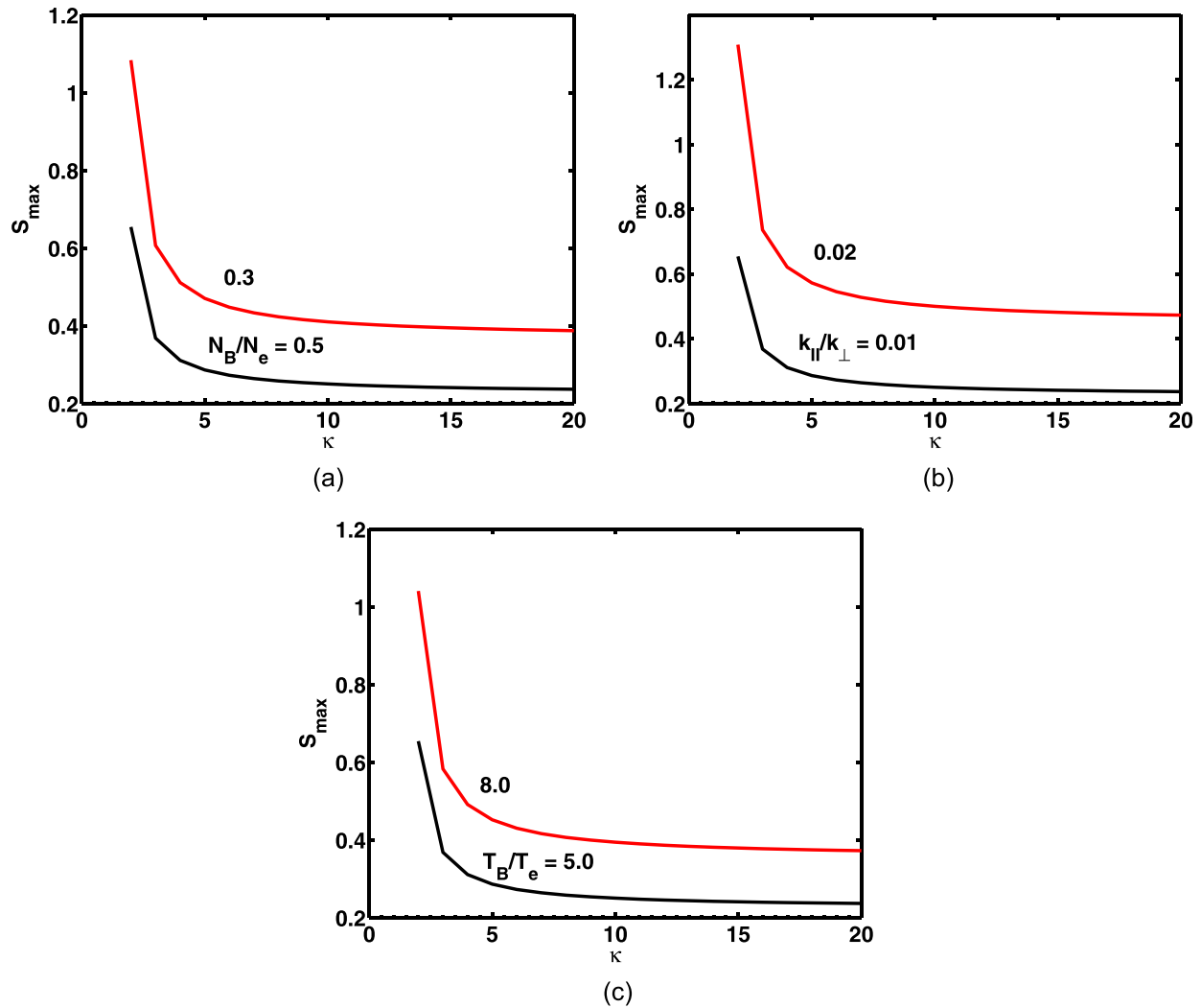
FIG. 1. KAWs Resonant instability driven by velocity shear: variation of velocity shear with the nonthermal index \kappa for (a) k_{\parallel}/k_{\perp} = 0.01 , T_B/T_e = 5.0 and N_B/N_e = 0.5, 0.3 , (b) N_B/N_e = 0.5 , T_B/T_e = 5.0 and k_{\parallel}/k_{\perp} = 0.01, 0.02 , and (c) N_B/N_e = 0.5 , k_{\parallel}/k_{\perp} = 0.01 and T_B/T_e = 5.0, 8.0 .
