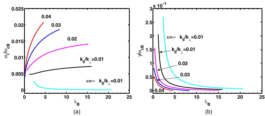
FIG. 6. KAW resonant instability driven by velocity shear: variation of (a) normalized real frequency, \omega_r/\omega_{cB} , and (b) normalized growth rate, \gamma/\omega_{cB} vs \lambda_B = \frac{k_{||}^2 \alpha_B^2}{2\omega_{cB}^2} for S = 0.5 , N_B/N_e = 0.3 , \beta_i = 0.001 , \kappa = 3, \infty and various values of k_{||}/k_{\perp} as listed on the curves.
