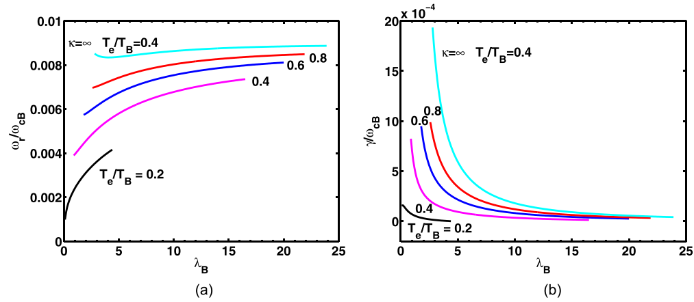
FIG. 7. KAW resonant instability driven by velocity shear: variation of (a) normalized real frequency, \omega_r/\omega_{cB} , and (b) normalized growth rate, \gamma/\omega_{cB} vs \lambda_B = \frac{k_{||}^2 \alpha_B^2}{2\omega_{cB}^2} for S = 0.3 , \kappa = 2, \infty , N_B/N_e = 0.3 , k_{||}/k_{\perp} = 0.01 , \beta_i = 0.001 and various values of T_e/T_B as listed on the curves.
