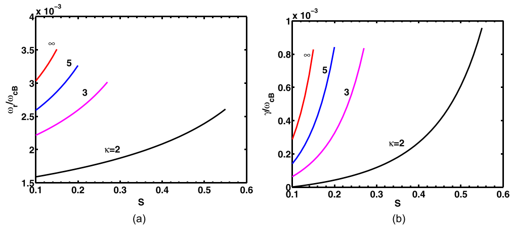
FIG. 4. KAW resonant instability driven by velocity shear: variation of (a) normalized real frequency, \omega_r/\omega_{cB} , and (b) normalized growth rate, \gamma/\omega_{cB} vs velocity shear S for N_B/N_e = 0.3 , \beta_i = 0.001 , k_{\parallel}/k_{\perp} = 0.01 , \lambda_B = 0.5 and various values of \kappa as listed on the curves.
