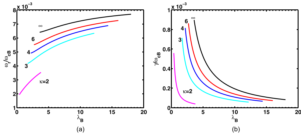
FIG. 2. KAW resonant instability driven by velocity shear: variation of (a) normalized real frequency, \omega_r/\omega_{cB} , and (b) normalized growth rate, \gamma/\omega_{cB} vs \lambda_B = \frac{k_{\perp}^2 \alpha_B^2}{2\omega_{cB}^2} for N_B/N_e = 0.5 , \beta_i = 0.001 , \frac{k_{\perp}}{k_{\parallel}} = 0.01 , S = 0.3 and various values of \kappa as listed on the curves.
