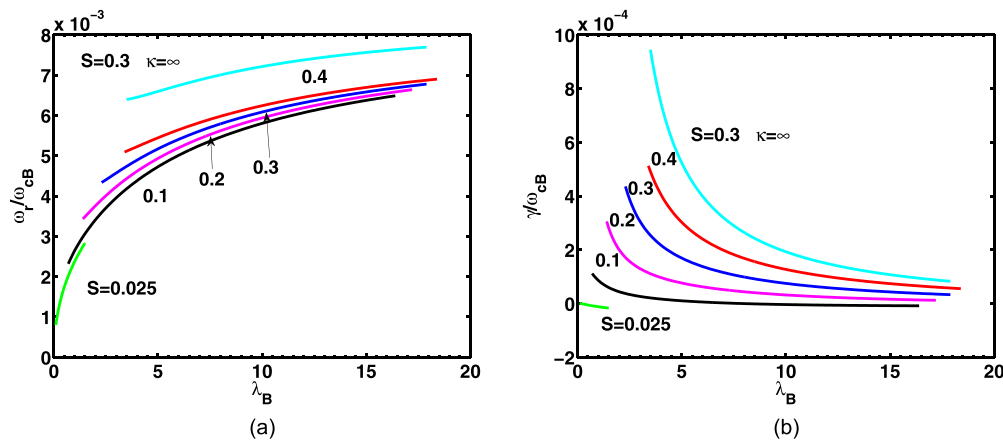
FIG. 3. KAW resonant instability driven by velocity shear: variation of (a) normalized real frequency, \omega_r/\omega_{cB} , and (b) normalized growth rate, \gamma/\omega_{cB} vs \lambda_B = \frac{k_{\perp}^2 \alpha_B^2}{2\omega_{cB}^2} for N_B/N_e = 0.5 , \beta_i = 0.001 , \frac{k_{\perp}}{k_{\parallel}} = 0.01 , \kappa = 3, \infty and various values of S as listed on the curves.
