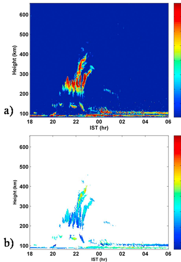
Figure 3. VHF radar observations for 23 March 2009: (a) range-time-intensity and (b) range-time-velocity.
