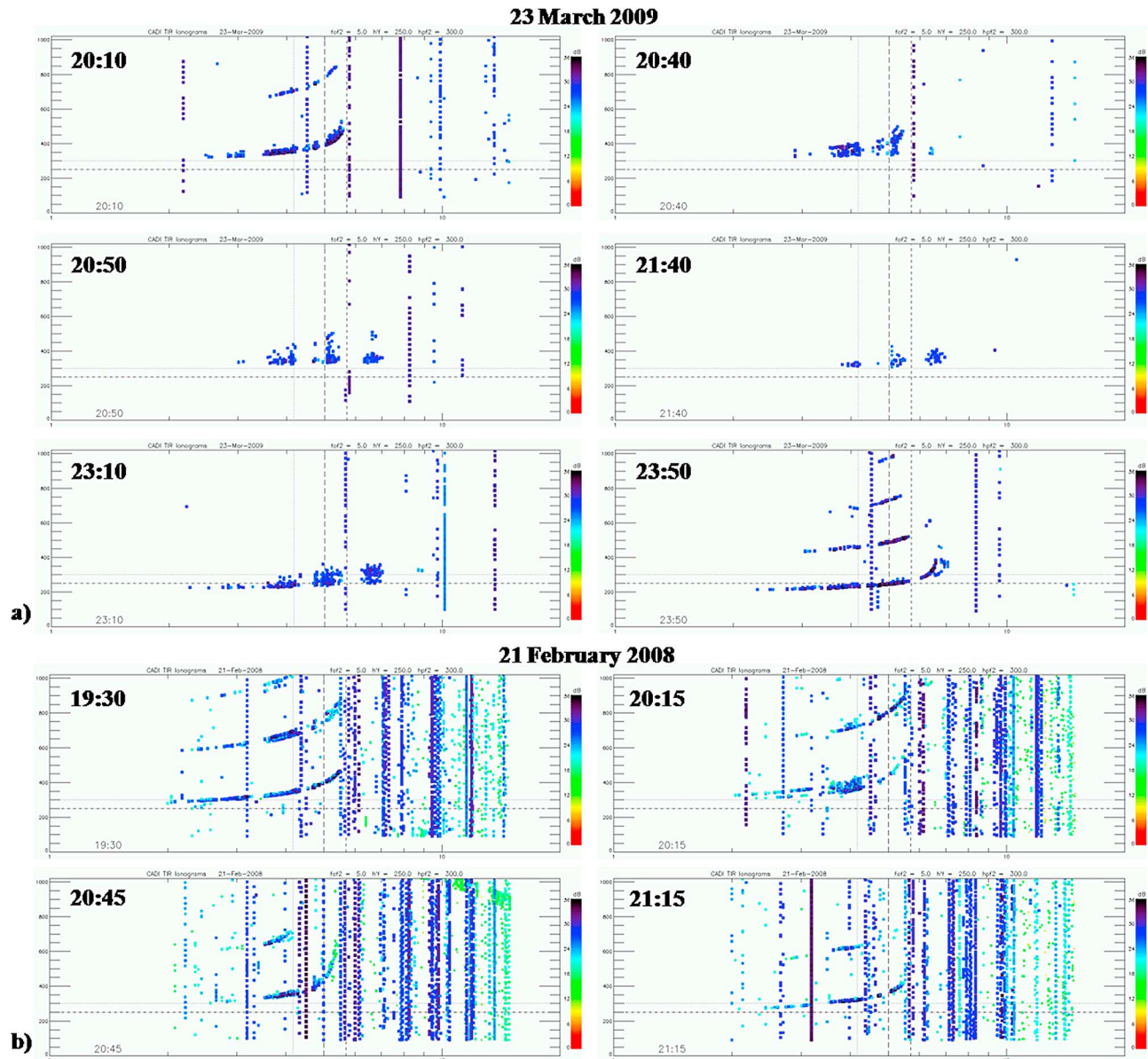
Figure 2. Ionograms recorded from the equatorial station Tirunelveli on the nights of (a) 23 March 2009 and (b) 21 February 2008. Times are in IST (UT + 5.5 h). The vertical lines are noise.
