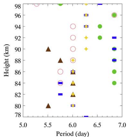
Figure 5. Periods of the maximum wavelet amplitudes over Yamagawa (blue solid square), Wuhan (green solid circle), Maui (yellow star), Tirunelveli (red open circle), and Adelaide (brown solid upward triangle).
