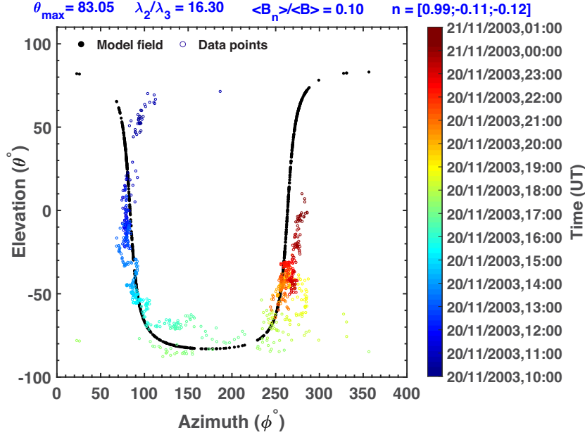
Figure 2. Distribution of azimuth ( \phi ) versus elevation ( \theta ) angle of the IMF in geocentric solar ecliptic coordinates. Note that \lambda_2/\lambda_3 , \langle B_n \rangle/B and n give information about the planarity, efficiency and normal direction of the PMS. \theta_{\max} is the inclination of the PMS plane with respect to the ecliptic plane. When IMF vectors \mathbf{B} = (B_x, B_y, B_z) \equiv (B \cos \theta \cos \phi, B \cos \theta \sin \phi, B \sin \theta) are parallel to a plane whose normal is \mathbf{n} \equiv (n_x, n_y, n_z) , the relation between \phi and \theta is given as n_x \cos \theta \cos \phi + n_y \cos \theta \sin \phi + n_z \sin \theta = 0 . The above curve fitting (see the black dotted curve) to the measured (coloured dots) \phi and \theta indicates the presence of PMS.
