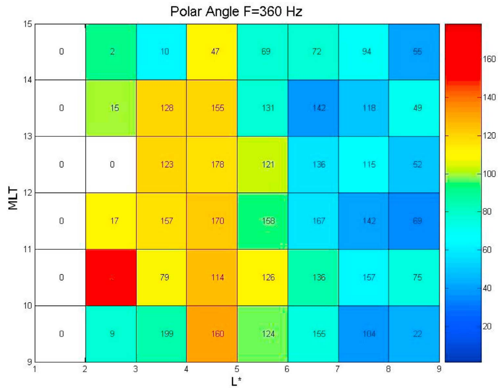
Figure 2. A distribution of wave Poynting vector polar angles as functions of MLT and L^* for \sim 360 Hz waves. The blue color for the bins indicates downgoing waves and orange and red indicate upcoming waves. Each \sim 2 min event was weighted by its log of the wave intensity to form the average polarization for each bin (the color). The number of \sim 2 min events is indicated in each box.
