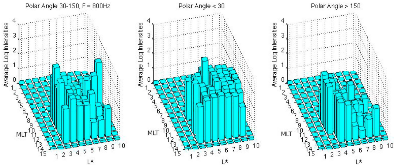
Figure 5. The spatial distribution of the log of the wave intensities for \sim 800 Hz waves. The log scale is given in the rear left of each panel. The scale has been shifted by 10^{-9} \text{ nT}^2 . (left) Oblique waves, (middle) parallel waves with \theta_{PB0} < 30^\circ and (right) waves with \theta_{PB0} > 150^\circ . Figures 5 (middle) and 5 (right) roughly correspond to blue and red waves, respectively.
