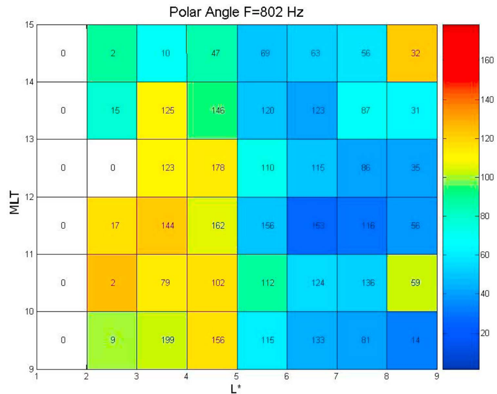
Figure 3. Same as for Figure 2, except for \sim 800 Hz waves.
