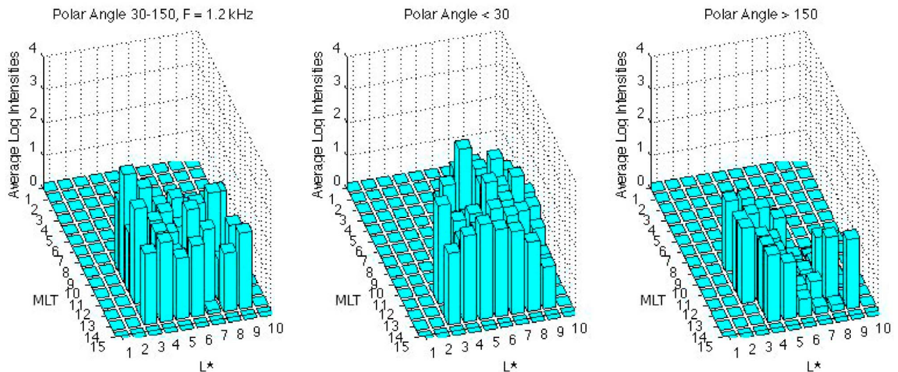
Figure 7. Same format as Figure 5, except for \sim 1.2 kHz waves.
