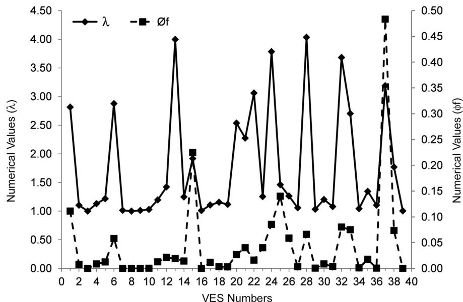
Fig. 9. Plot of coefficient of anisotropy ( \lambda ) and fracture porosity ( \phi_f ) with VES numbers.
