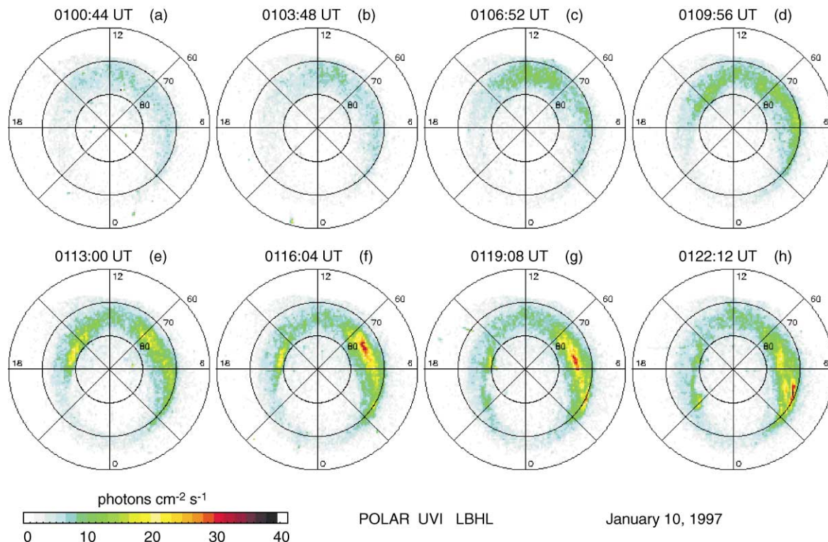
Fig. 2. POLAR UV images of the dayside aurora prior to and after shock compression of the magnetosphere. The time sequence goes from left to right and down. A magnetic coordinate system is used with magnetic local noon at the top and dawn at the right of the images. The linear color scale indicates the photon flux ( \text{photons cm}^{-2} \text{s}^{-1} ) collected in the instrumentation aperture due to optical emission within a single pixel at the emission region.
