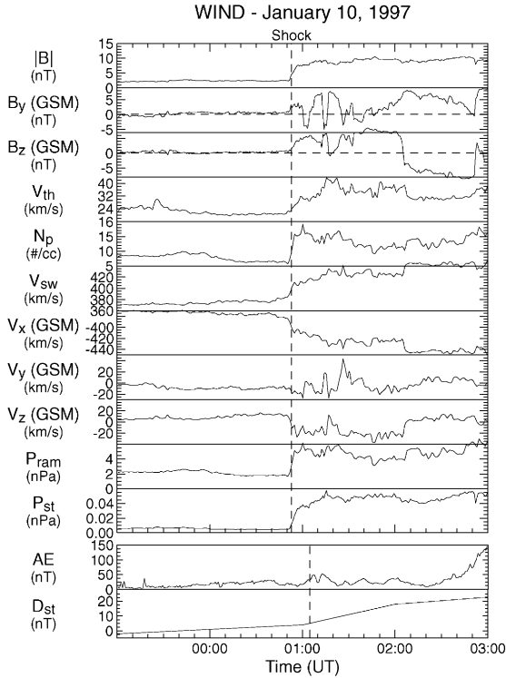
Fig. 1. The January 10, 1997 interplanetary shock events. An interplanetary shock is observed by WIND at 0052 UT (the dashed line). At the time, WIND was located at (85, -59, -3) R_E upstream of the Earth in GSE coordinates.
