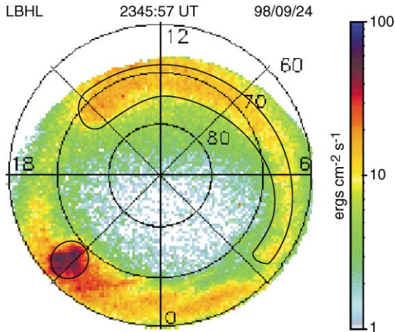
Fig. 6. The dayside aurora and a nightside substorm. The total dayside energy disposition rate is \sim 3 – 4 times that of the substorm.
