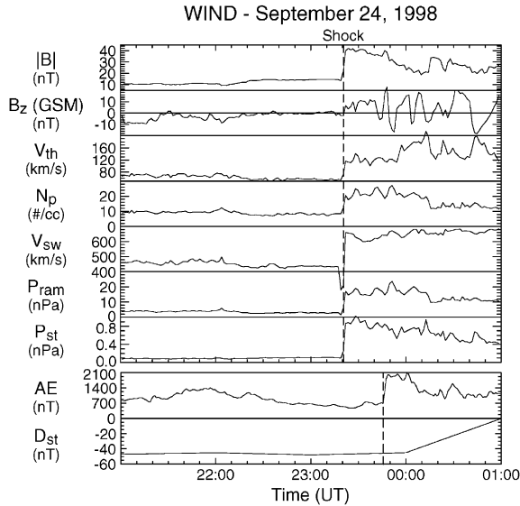
Fig. 4. The interplanetary shock of September 24, 1998. The IP shock is observed by WIND at 2320 UT at (183, 15, -6)R_e upstream of the Earth in GSE coordinates.
