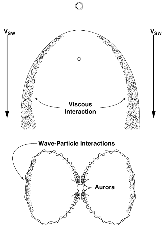
Fig. 10. A schematic representation of viscous interaction.
