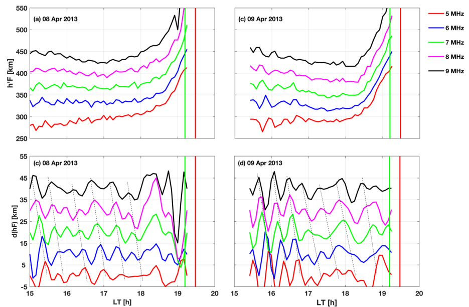
Figure 7. Temporal variations in the fixed frequency (5–9 MHz) virtual heights ( h'F ) (upper panel) and virtual height deviations ( dh'F , band-pass filtered between 20 and 90 min) (lower panel) observed at Chumphon during 15–20 LT on 8 and 9 April 2013. The black dotted lines indicate the downward phase propagation of GW. The green and red lines indicate the E region and F region sunset over Chumphon.
