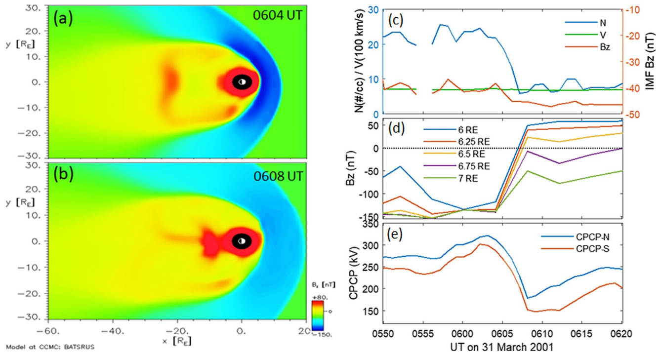
Figure 4. Results of magneto-hydro-dynamic (MHD) simulation using the Block-Adaptive-Tree-SolarWind-Roe-Upwind-Scheme model coupled with the Ring Current Model. Panels (a) and (b) show the variation of Bz in the GSM-XY plane during 0604 and 0608 UT, respectively. (c) Variations of upstream solar wind velocity (green), density (blue), and IMF Bz measured at L1-point. (d) Bz variations at 6–7 Re from the MHD simulation. (e) Cross polar cap potential (CPCP) variations at Northern and Southern Hemispheres as a function of UT.
