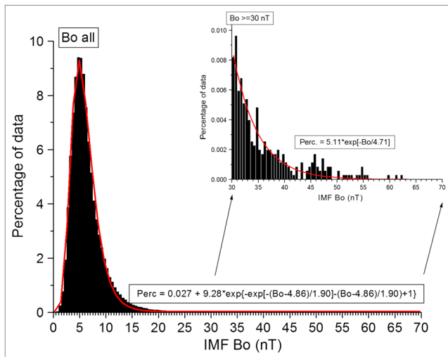
Figure 2. Same format as in Figure 1 but for the interplanetary magnetic field magnitude B_0 . A blowup of the magnetic field between 30 nT and 70 nT is given in the inset.
