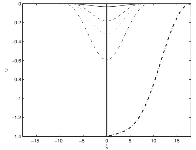
FIG. 5. Nonlinear wave structures: Variation of electrostatic potential \psi vs \xi for \tau = 0.04 , f = 0.1 , M = 0.98 , \theta = 15^\circ (—), \theta = 25^\circ (---), \theta = 30^\circ (···), \theta = 35^\circ (-.-), and \theta = 38.0425^\circ (*) (double layer)
