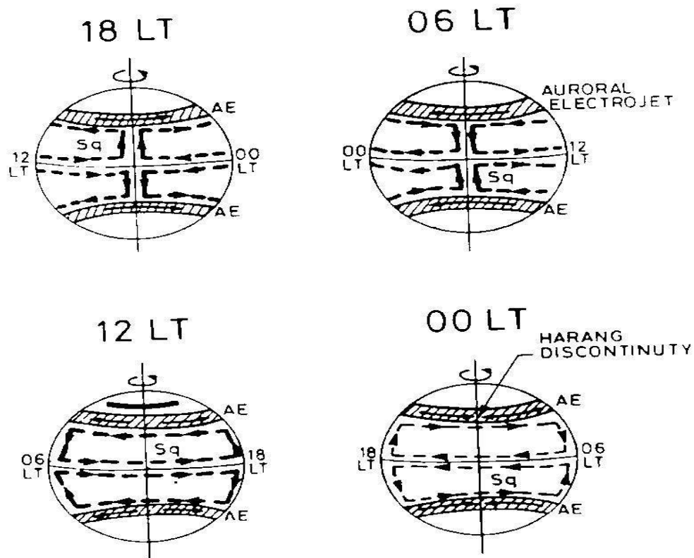
Fig. 11 Current systems influencing high latitude quiet times
