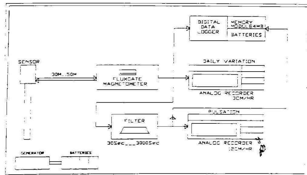
Fig. 3. Block diagram of Fluxgate Magnetometer set-up used to record daily variations and pulsations in the X, Y & Z components of the geomagnetic field at Maitri & Dakshin Gangotri
