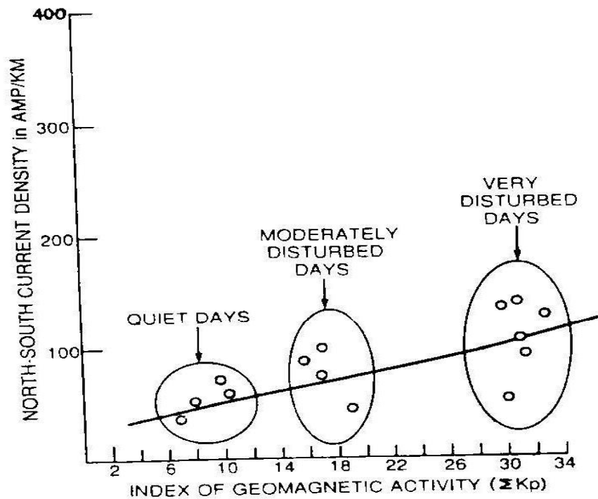
Fig.9: Variation of North-South Ionospheric Current Density i_x (in amp/Km) with index of Geomagnetic Activity ( k_p ) for Dusk Sector at Maitri during January 1994
