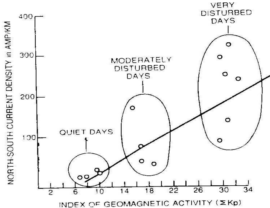
Fig. 7 Variation of North-South Ionospheric Current Density i_x (in amp/Km) with index of Geomagnetic Activity ( k_p ) for Dawn Sector at Maitri during January 1994
