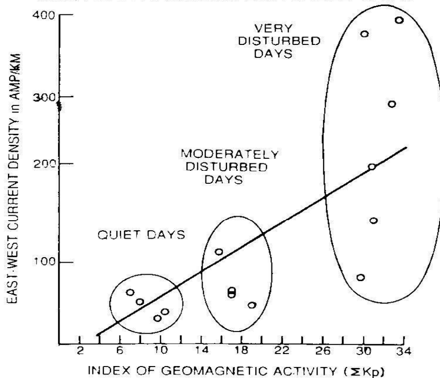
Fig. 8: Variation of East-West Ionospheric Current Density i_y (in amp/Km) with index of Geomagnetic Activity ( k_p ) for Dawn Sector at Maitri during January 1994
