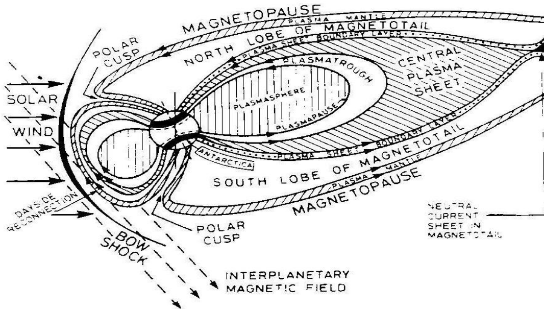
Fig.1: Polar cross-section of Earth's magnetosphere as viewed from a point in space in the duskside. The Central Plasma sheet region of the magnetosphere maps into the auroral regions of the Earth
