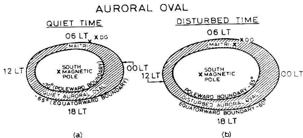
Fig. 2: The auroral oval during magnetically quiet times usually lies between 65^\circ and 70^\circ latitudes. At is always a little broader and more pulled away from the magnetic pole towards the nightside. At such times, the Indian Antarctic station, Maitri & DG lie just equatorwards of the auroral oval as shown in Fig. 2(a). During magnetic disturbance, both the stations move into the auroral oval as shown in Fig. 2(b). The auroral oval occupies the latitudinal region 60 - 65^\circ because of moves equatorward during disturbances
