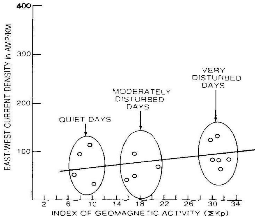
Fig. 10: Variation of East-West Ionospheric Current Density i_y (in amp/Km) with index of Geomagnetic Activity ( k_p ) for Dusk Sector at Maitri during January, 1994
