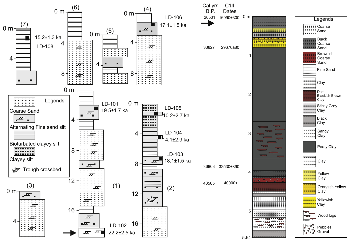
Fig. 4. Lithology of the sediment profiles from Ziro valley as in Srivastava et al. (2009) modified and compared with the lithology of the present sediment profile (shown in color) from Ziro valley Arunachal Pradesh. (For interpretation of the references to color in this figure legend, the reader is referred to the web version of this article.)
