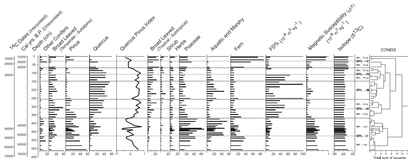
Fig. 8. Diagram showing Quercus – Pinus Index, Magnetic Susceptibility, \delta^{13}\text{C} Isotope variations in the sediment profile and its comparison with major palynomorphologic elements which comprise the vegetation in Ziro valley Arunachal Pradesh.
