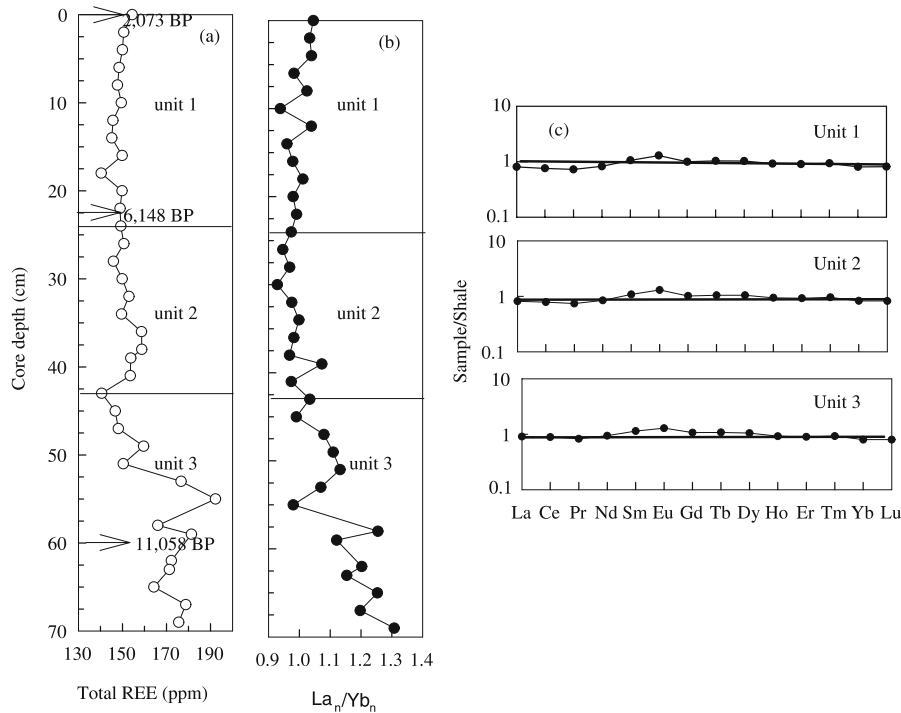
Figure 7. Down-core REE variations: (a) total REE, (b) \text{La}_n/\text{Yb}_n , and (c) shale normalized average REE patterns in three units. Observe a change in the \text{La}_n/\text{Yb}_n ratios between unit 3 and in units 2 and 1 suggesting a change in the provenance.
