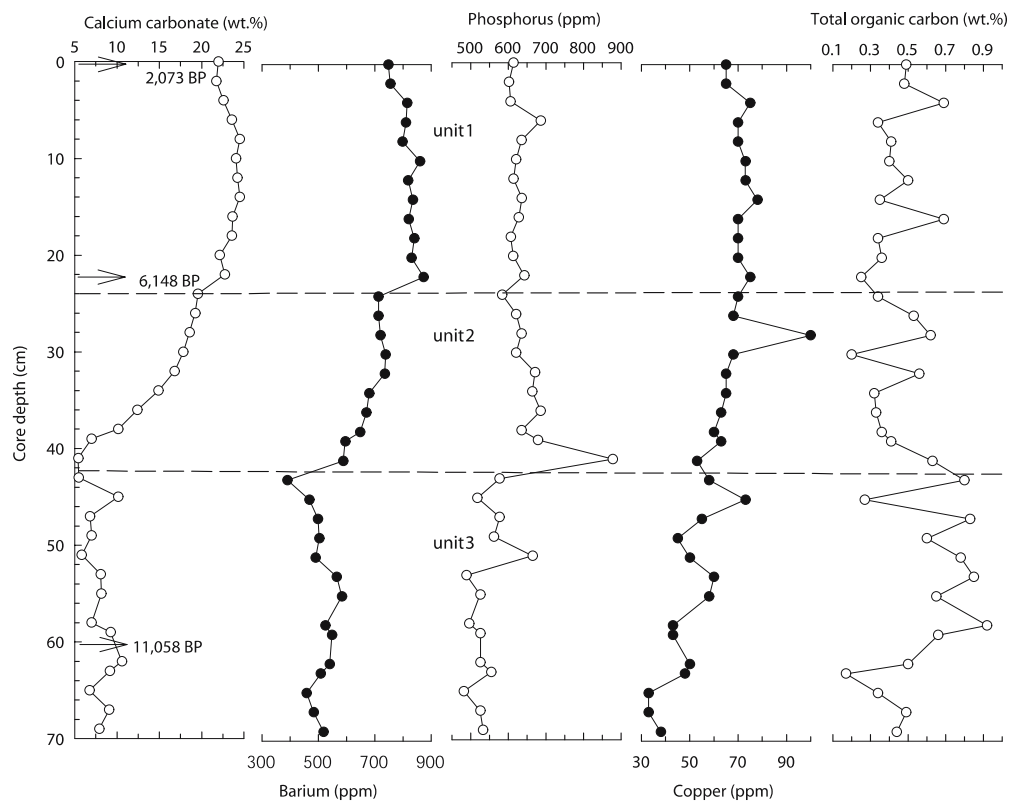
Figure 4. Down-core variations of biogenic elements CaCO 3 , Ba, P, Cu and total organic carbon (TOC). Note the accumulation of biogenic elements in unit 1.
