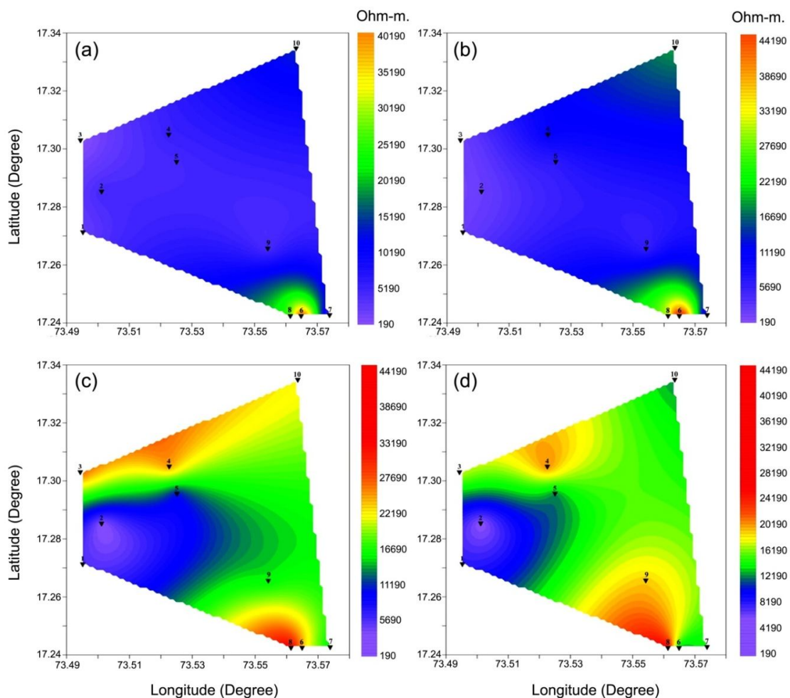
Figure 4 (a-d): Apparent resistivity distribution at various depths (a- 1m, b-2m, c-10m, d-20m).
