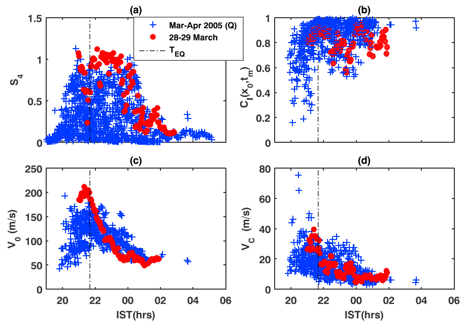
Figure 3. Variation of (a) S_4 index, a measure of strength of scintillation, (b) maximum cross correlation between two spaced receivers C_l(x_0, t_m) , (c) zonal irregularity drift V_0 , and (d) random velocity V_c are plotted as a function of IST for quiet days of March–April 2005 (blue color) and earthquake day 28 March 2005 (red color). The time of start of earthquake T_{EQ} is shown by vertical dash-dotted lines in all subplots. IST = Indian standard time.
