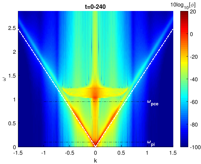
FIG. 3. \Omega - k dispersion diagram obtained from the electrostatic potential during t = 0 –240 of run-1. It shows the presence of both Langmuir and electron acoustic modes. The speed of electron acoustic mode ( V_s = 1.65 ) estimated from its standard linear dispersion equations is shown with the slanted dashed-dotted lines. The cold electron (ion) plasma frequency is shown with a horizontal black line at \omega_{pce} = 0.95 ( \omega_{pi} = 0.1 ).
