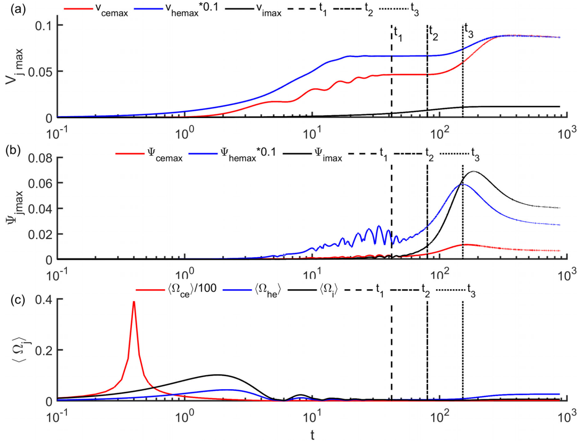
FIG. 7. Variation of (a) maximum velocities ( V_{jmax} ), (b) maximum ponderomotive potentials ( \Psi_{jmax} ), and (c) ponderomotive frequencies ( \Omega_i ) of the cold electron, hot electron, and ion with time for run-1. The vertical dashed, dashed-dotted, and dotted lines represent the time of formation of two EA pulses (at t_1 = 46 ), time of initiation of wave steepening (at t_2 = 80 ), and time of wave breaking (at t_3 = 152 ) for run-1, respectively.
