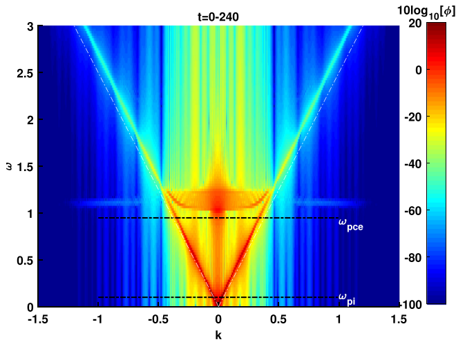
FIG. 5. \Omega - k dispersion diagram obtained from the electrostatic potential during t=0 –240 of run-3. It shows the presence of both Langmuir and electron acoustic modes. The speed of electron acoustic mode ( V_s = 2.5 ) estimated from its standard linear dispersion equations is shown with slanted white dashed lines. The cold electron (ion) plasma frequency is shown with a horizontal black line at \omega_{pce} = 0.95 ( \omega_{pi} = 0.1 ).
