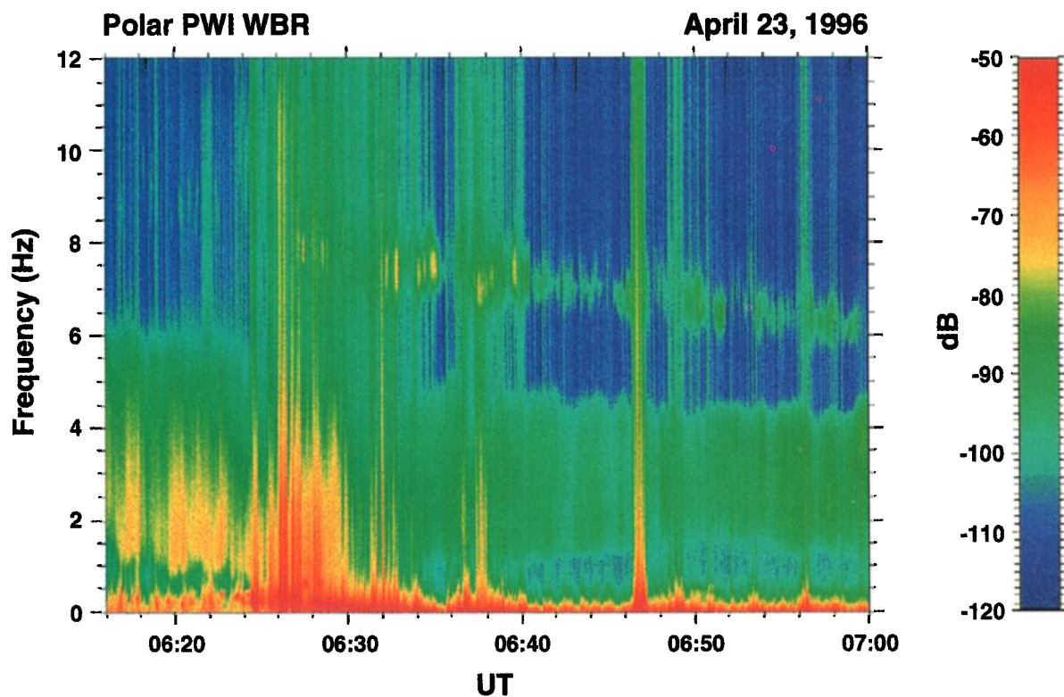
Plate 2. Wideband high time resolution plot for the PCBL wave event on Day 114, 1996. The waves are very spiky and highly variable in intensity.
