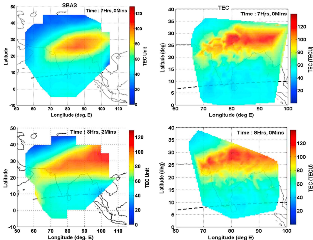
Figure 9. A comparative study of the ionospheric TEC maps generated from (left) SBAS broadcast iono corrections from a single SBAS receiver, and from (right) a dense network of dual-frequency receivers (GAGAN-TEC Network) at different times on 29 September 2012, depicting the development of strong EIA. The horizontal dashed line passing through the southern tip of India is magnetic equator. The fairly good agreement in both contours highlights the potential of using a single-SBAS receiver data.
