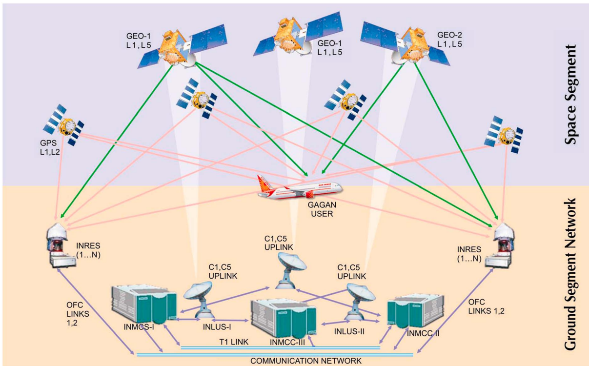
Figure 2. Configuration of Indian SBAS-GAGAN (Courtesy AAI/ISRO). GAGAN consists of 15 reference stations (INRES), 3 Master control centers (INMCC) and 3 Uplink stations (INLUS).
