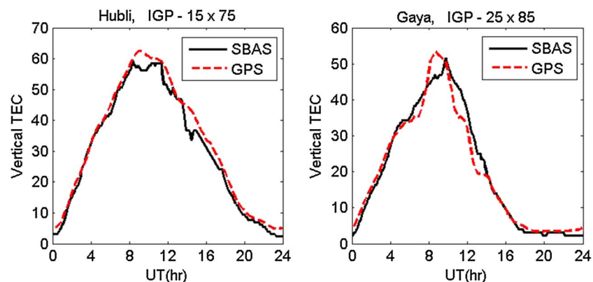
Figure 8. Comparison of vertical TEC derived from GPS measurements (dashed line) and SBAS (GAGAN) corrections (solid line) at two different locations—(left) Hubli (15.3°N, 75°E) and (right) Gaya (24.75°N, 84.95°E) on a typical day of 23 November 2012.
