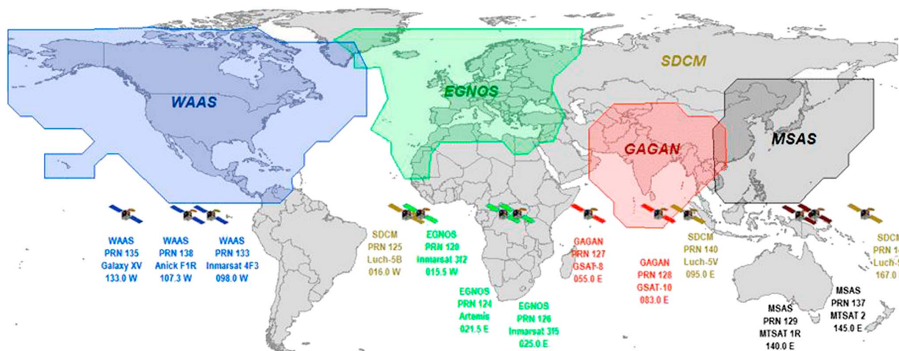
Figure 1. Fleet of operational SBAS-GEO satellites along with marked service area of each SBAS around the globe. The PRN and location of each GEO satellite is also indicated on the map. (Courtesy GENEQ Inc.)
