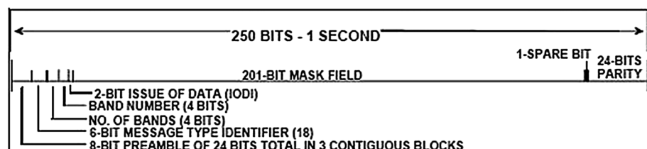
Figure 4. Message Type 18 IGP mask message format (Courtesy RTCA/DO-229B).
