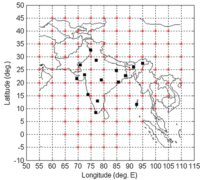
Figure 5. Ionosphere grid points (IGPs) served by GAGAN system (denoted by stars) and the location of 15 GAGAN reference stations marked by squares.
