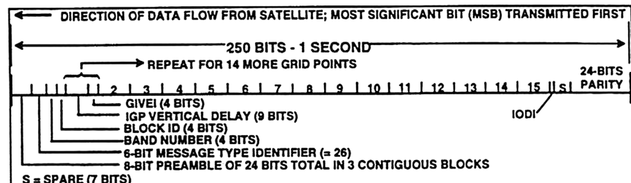
Figure 6. Message type 26 ionospheric delay corrections message format (Courtesy RTCA/DO-229B).
