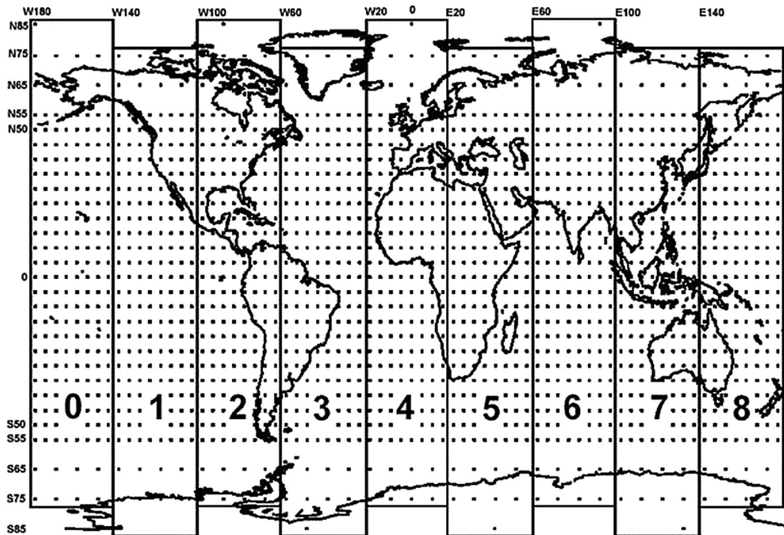
Figure 3. Predefined global ionospheric grid points (IGPs). The bold numbers in rectangular shape denote the band numbers (Courtesy RTCA/DO-229B).
