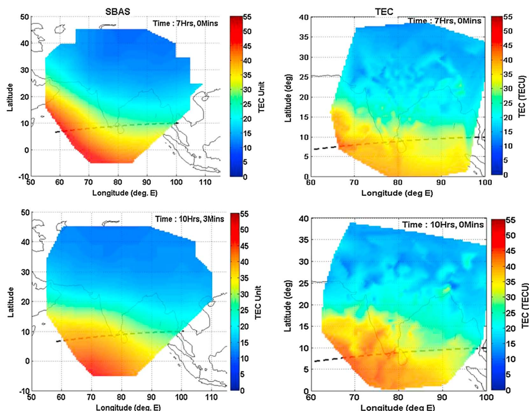
Figure 10. Comparative study of the regional TEC maps developed from (left) SBAS iono corrections and (right) TEC measurements from 23 stations (GAGAN-TEC network) at different times on 16 July 2012 in the wake of a geomagnetic storm, i.e., during the recovery phase of a geomagnetic storm. The horizontal dashed line passing through the southern tip of India is magnetic equator. The behavior of the ionosphere during such dynamic space weather events could be studied with unprecedented spatial and temporal resolution.
