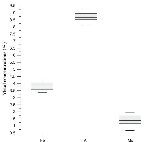
Figure 9. Box-whisker plot of Fe, Al and Mg concentrations in Chennai coastal sediments.
