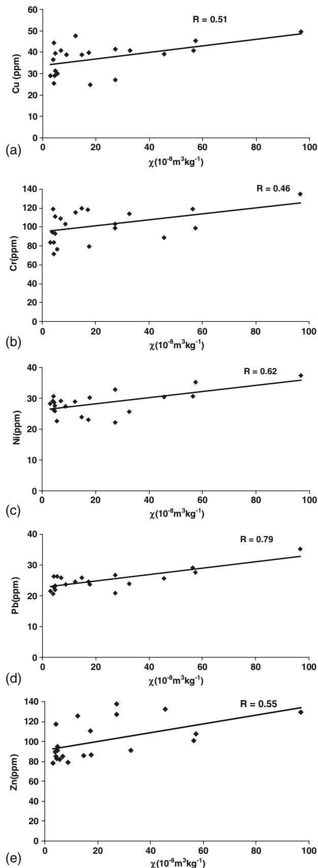
Figure 12. (a–e) Plot of Cu, Cr, Ni, Pb and Zn vs. \chi in Chennai coastal sediments.
