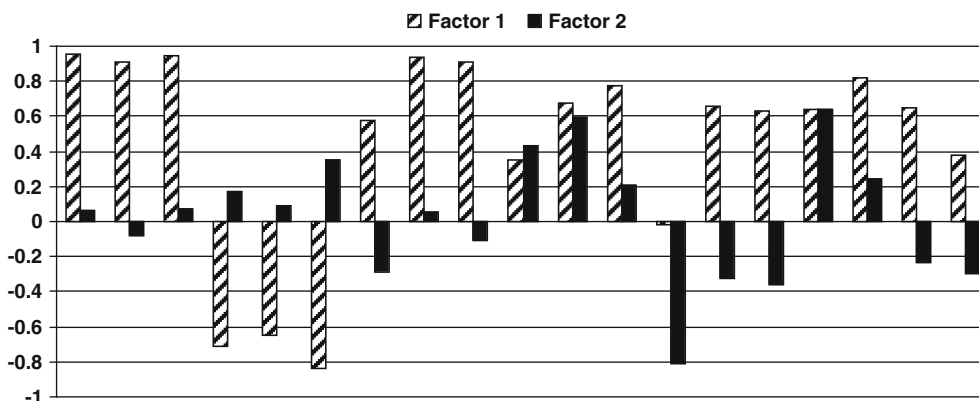
Figure 14. Results of factor analysis (R-mode) showing the association of the two primary factors for Chennai coastal sediments.
