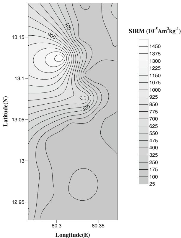
Figure 4. Contour plot of spatial distribution of saturation isothermal remanent magnetization of the Chennai coastal sediments.
