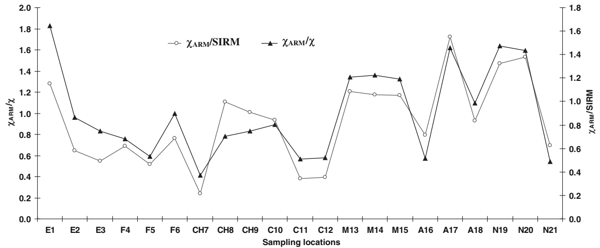
Figure 7. Spatial distributions of magnetic carrier dependent parameter ratios ( \chi_{\text{ARM}}/\chi and \chi_{\text{ARM}}/\text{SIRM} ).
