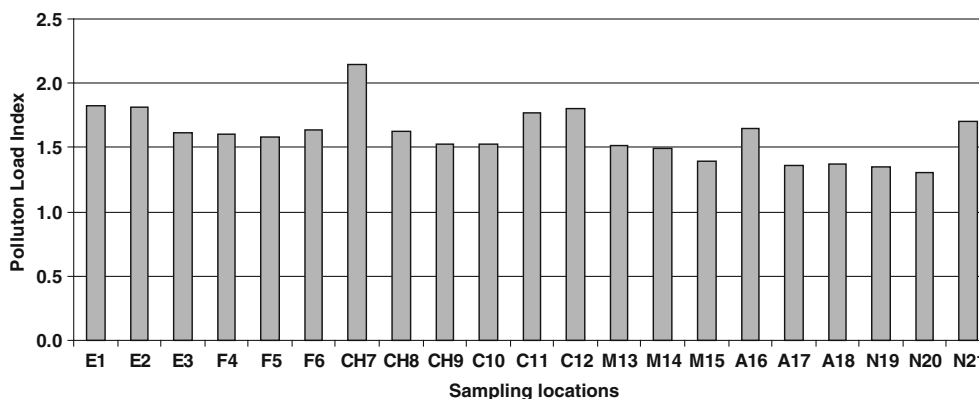
Figure 11. Pollution load index of Chennai coastal sediments.
