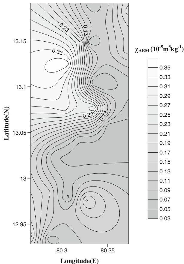
Figure 3. Contour plot of spatial distribution of susceptibility of anhysteretic remanent magnetization of the Chennai coastal sediments.
