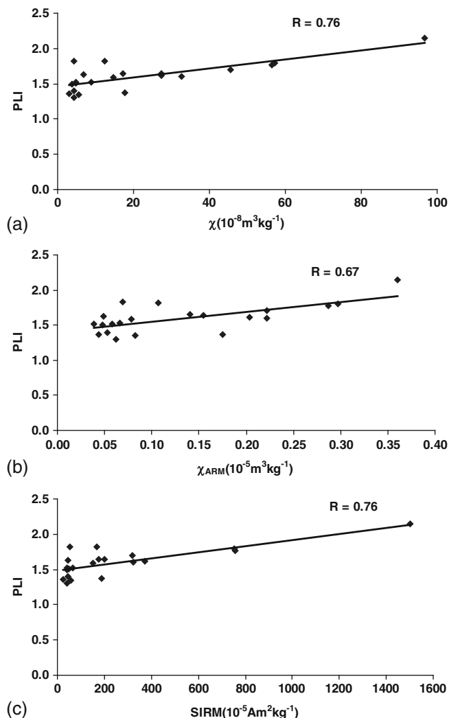
Figure 13. (a–c) Plot of \chi , \chi_{\text{ARM}} and SIRM vs. PLI in Chennai coastal sediments.
