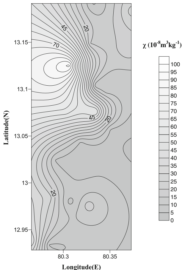
Figure 2. Contour plot of spatial distribution of magnetic susceptibility of the Chennai coastal sediments.
