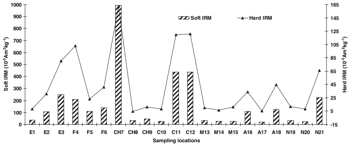
Figure 6. Spatial distribution of soft and hard IRMs in Chennai coastal sediments.
