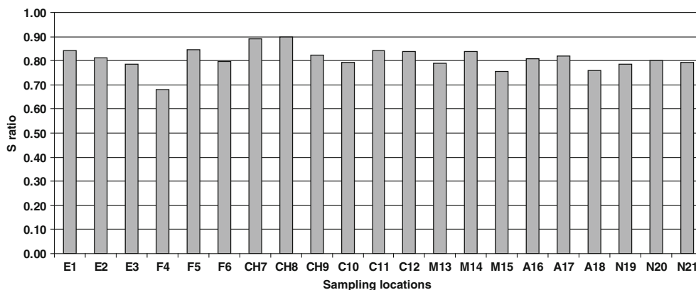
Figure 5. Spatial variation of S ratio in Chennai coastal sediments.
