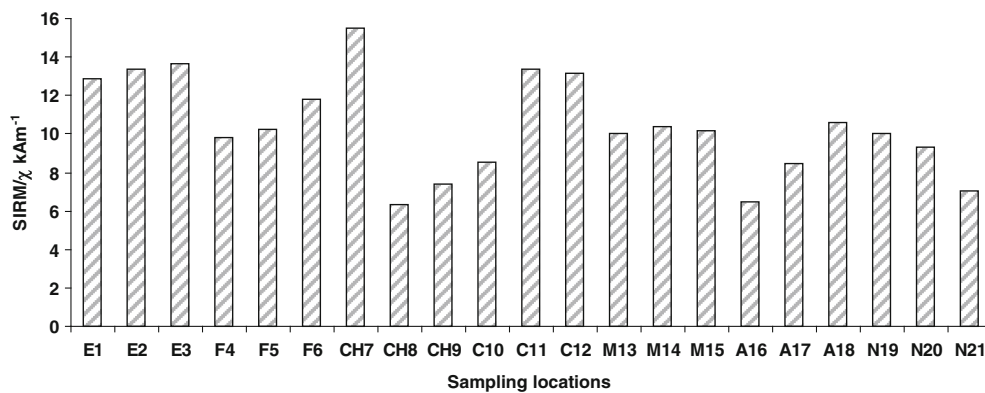
Figure 8. Spatial variation of SIRM/ \chi ratio in Chennai coastal sediments.
