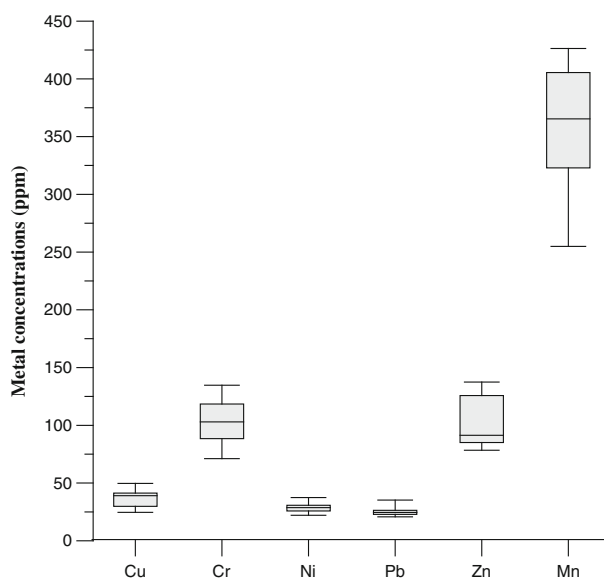
Figure 10. Box-whisker plot of Cu, Cr, Ni, Pb, Zn and Mn concentrations in Chennai coastal sediments.
