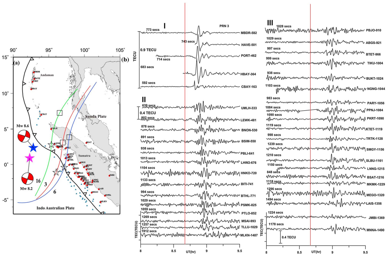
Figure 1. (a) Locations of GPS stations of Sumatra and Andaman used in the present study. GPS sites are marked by the red solid circles, and the SIPs of satellite 3 are marked by blue triangles. The colored stars show the epicenters of the main shock ( M_w 8.6) and aftershock ( M_w 8.2), respectively. Red, blue, and green solid curves represent the trajectories of satellites 3, 6, and 16, respectively. Black open stars along the trajectories are the SIPs of the CID arrival for the main shock at site LEWK. Black open squares along the trajectories are SIPs at the time of aftershock at 10:43 (UTC). Beach balls indicate the focal mechanism of two earthquakes. (b) Traces of band pass-filtered (1–10 min) coseismic TEC variation as observed by GPS satellite PRN 3. The vertical line indicates the origin time of the main shock. Distances of the SIPs of GPS sites from the epicenter are indicated on the right side and on the left side is the CID arrival time at that particular site after the earthquake.
