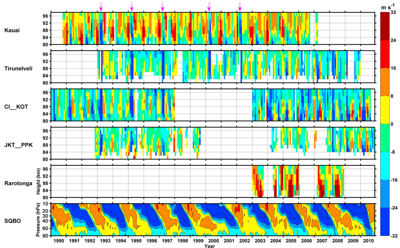
Figure 2. Height-month contours of monthly mean zonal winds for Kauai, Tirunelveli, Christmas Island and Koto Tabang (CI KOT), Jakarta and Pameungpeuk (JKT_PPK), and Rarotonga (first through fifth panels). The sixth panel shows the monthly winds associated with stratospheric quasi biennial oscillation (SQBO).
