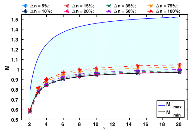
FIG. 6. Variation of Mach numbers with \kappa . The solid black line represents the lower ( M_{\min} ) and the solid blue line represents the upper ( M_{\max} ) Mach number limit predicted by nonlinear fluid theory for the existence of the IA solitons. Shaded region shows Mach number range for the existence domain of the IA solitons predicted by the nonlinear fluid theory. The different asterisk color points are the Mach numbers obtained from the simulation for different combinations of kappa and the amplitude of the IDP.
