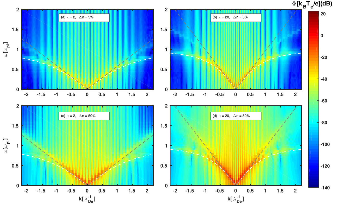
FIG. 3. \omega - k diagram during \omega_{pi}t = 0 - 200 for simulation runs: (a) Run-1(I), (b) Run-1(VII), (c) Run-6(I), and (d) Run-6(VII). The dashed gray lines are from the linear dispersion of the IA waves which is derived by considering plasma quasi-neutrality approximation, whereas white dashed lines are from the dispersion relation of IA waves which is derived without consideration of the plasma quasi-neutrality approximation.
