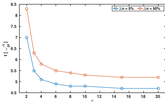
FIG. 5. The variation of the IASW pulse formation time (see Figure 2(c)) with the kappa index. The blue color is for the perturbation \Delta n = 0.05 and the red color lines represent the case of the \Delta n = 0.5 perturbation in ion and electron equilibrium densities.
