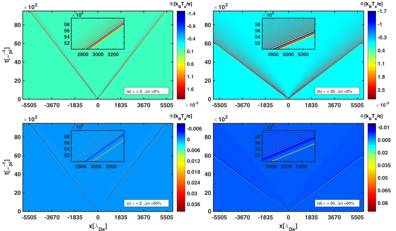
FIG. 2. Spatiotemporal evolution of the electrostatic potential in the system for different combination of \kappa and \Delta n : (a) Run-1(I), (b) Run-1(VII), (c) Run-6(I), and (d) Run-6(VII). In all the four plots, intense red band is due to the IASW pulse and the other alternate blue and light red color bands are due to the IA oscillations.
