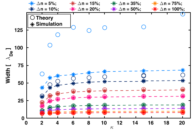
FIG. 8. Figure shows the variation of the maximum full width at half maximum for different combinations of the \kappa and IDP amplitude. The circles represent the \Phi_{\max} obtained from the theory, whereas the asterisks represent the soliton widths obtained from the simulation.
