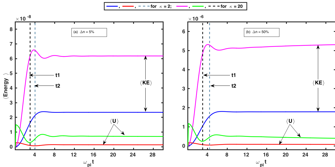
FIG. 4. The evolution of the average electrostatic energy \langle U \rangle and kinetic energy \langle KE \rangle of the ions in the system for the different kappa index and the amplitude of IDP for the runs discussed in Figure 2. The vertical dashed lines at time t_1 (for \kappa=20 ) and t_2 (for \kappa=2 ) show the time at which the trough formation begins at the top point of the potential pulse.
