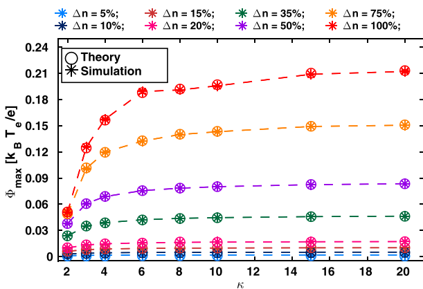
FIG. 7. Figure shows variation of the maximum electrostatic potential supported for different \kappa values and the different amplitude of the IDP. The circles represent the \Phi_{\max} obtained from the theory, whereas the asterisks represent the \Phi_{\max} obtained from simulation.
