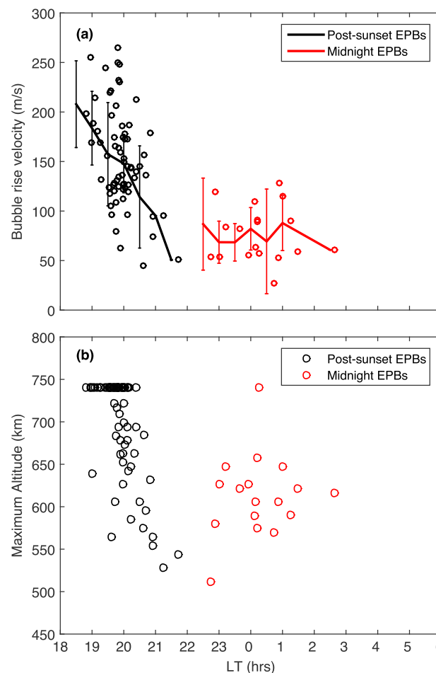
Figure 5. Local time variation of the (a) vertical rise velocity ( V_r ) and (b) maximum attainable altitude ( H_m ) of postsunset (black circles) and midnight (red circles) EPBs observed from the EAR.
