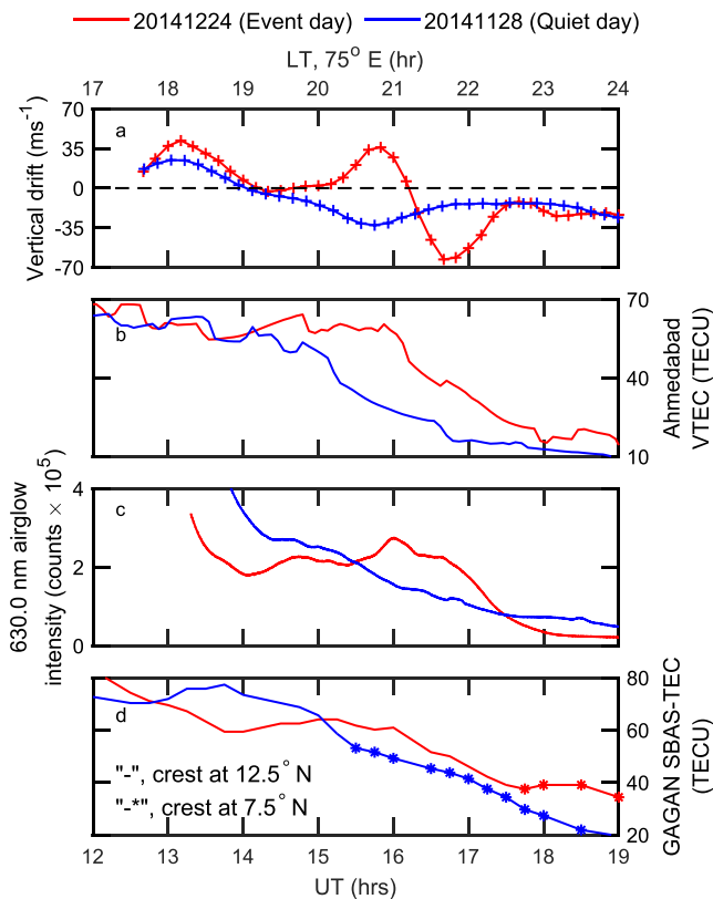
Figure 2. This figure illustrates the variations of a number of parameters on the event day (24 December 2014) and quiet day (28 November 2014) with red and blue colors, respectively. Subplots (a–d) represent vertical drifts (in \text{m s}^{-1} ) over Tirunelveli, vertical total electron content (in TECU) over Ahmedabad, OI 630.0 nm airglow intensity (in arbitrary unit) over Mt. Abu, and SBAS-TEC (in TECU) variations over only the crest location, respectively. In subplot (d), solid and solid lines with stars are used to show the position of the crest at 12.5^\circ\text{N} and 7.5^\circ\text{N} magnetic latitudes.
