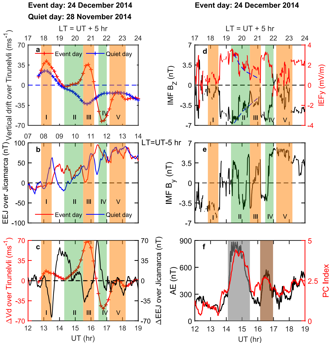
Figure 3. (a) The comparison of vertical drifts over Tirunelveli on the event day (24 December 2014, in red) with respect to a typical quiet day (28 November 2014, in blue) similar to what is shown in Figures 2a and 2b represents similar comparison in equatorial electrojet (EEJ) over Jicamarca, (c) shows the variations in the \Delta Vd over Tirunelveli (in red) and \Delta EEJ over Jicamarca (in black) obtained by subtracting the quiet day variation from the event day variation, (d) depicts the variations in interplanetary magnetic field (IMF) B z (in black) and IEFy (in red), (e) represents the variations in IMF B y and, (f) depicts the variations in the AE (in black) and PC (in red) indices. Based on vertical drift variations on event day, intervals (I–V) are marked with orange and green colored rectangular boxes in the panels (a–e). In (e), two conspicuous peaks in the AE and PC indices are marked with gray and brown colored rectangular boxes.
