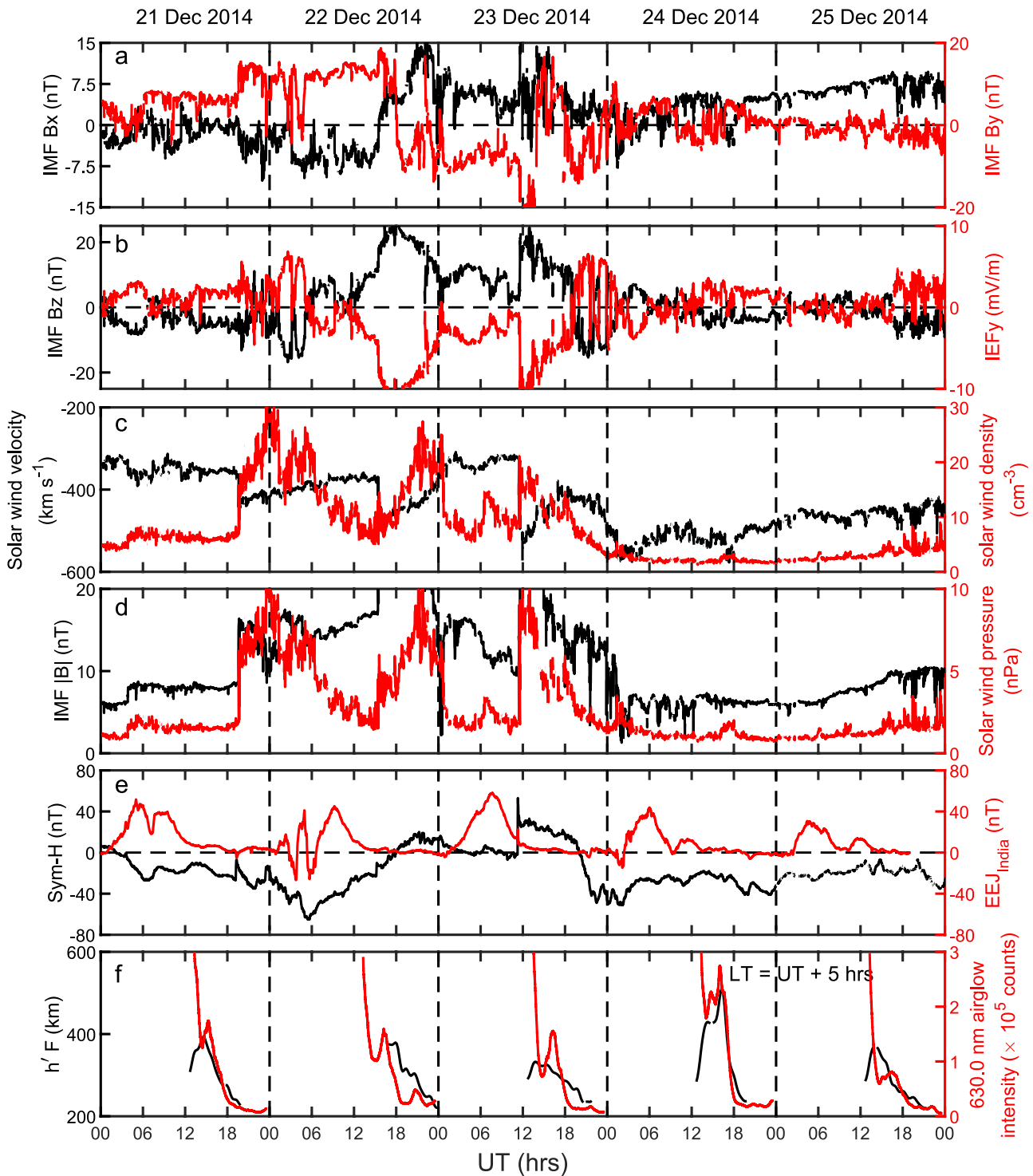
Figure 1. Variations in (a) interplanetary magnetic field (IMF) Bx (nT, black line) and IMF By (nT, red line), (b) IMF Bz (nT, black line) and IEFy (mV/m, red line), (c) solar wind velocity ( \text{km s}^{-1} , black line) and density ( \text{cm}^{-3} , red line), (d) IMF |B| (nT, black) and pressure (nPa, red), (e) Sym-H index (nT, black) and equatorial electrojet strength ( \text{EEJ}_{\text{India}} ) over the Indian sector (nT, red), (f) h'F (km, black) and OI 630.0 nm airglow intensity over Mt. Abu (in arbitrary units, red) from 21 December 2014 to 25 December 2014.
