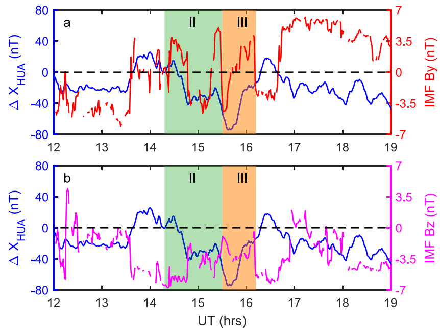
Figure 7. Variations in \Delta X over Huancayo (HUA) on 24 December 2014 is shown with blue colored line in panels a and b similar to Figure 5d. Variation in interplanetary magnetic field (IMF) B_y (in red) and IMF B_z (in magenta) are superimposed on the variations \Delta X in panels a and b, respectively. The intervals II and III are also marked similar to Figure 3.
