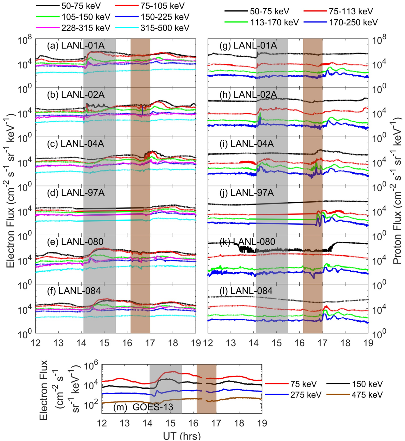
Figure 4. (a–f) and (g–l) The electron and proton flux variations measured by six LANL satellites (LANL-01A, LANL-02A, LANL-04A, LANL-97A, LANL-080, LANL-084) during 12:00–19:00 UT on 24 December 2014 for a number of energy channels mentioned at the top. (m) The electron flux variations at four energy channels (75, 150, 275, 475 keV) measured by GOES-13 for same interval and day depicted in (a–l). Two intervals are marked with gray (~14:05–15:30 UT) and brown (~16:10–17:00 UT) rectangular boxes in all subplots, similarly marked in Figure 3f.
