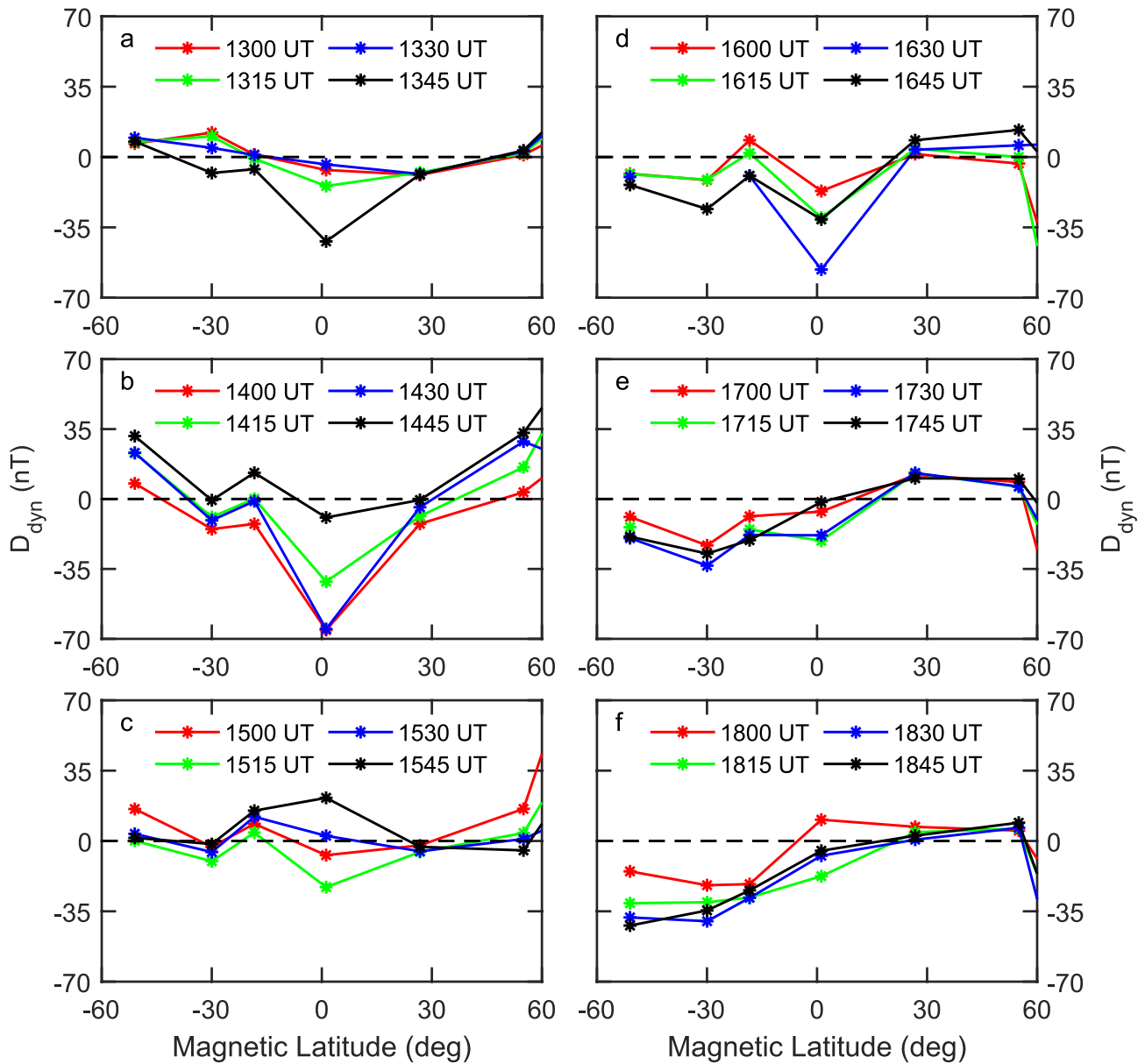
Figure 6. (a–f) The latitudinal variations in D_{dyn} during 13:00–18:45 UT in steps of 15 min intervals along Jicamarca longitudes on 24 December 2014. It can be seen that the positive deviations in D_{dyn} over equatorial latitudes are seen during 15:30–15:45 UT (in (c)) and 18:00 UT (in (f)) indicating influence of disturbance dynamo effects.
