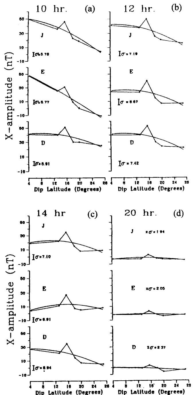
Figure 4. Variations of X amplitudes and their second-order polynomial fit obtained with dip-latitude for (a) 1000 LT, (b) 1200 LT, (c) 1400 LT and (d) 2000 LT. The vertical bars in each of the figures depict the magnitude of the standard deviation ( \sigma ). Note that the deviation of the amplitudes from the best-fit curve at the latitude of NAG is almost twice that of the standard error at all the selected hours.
