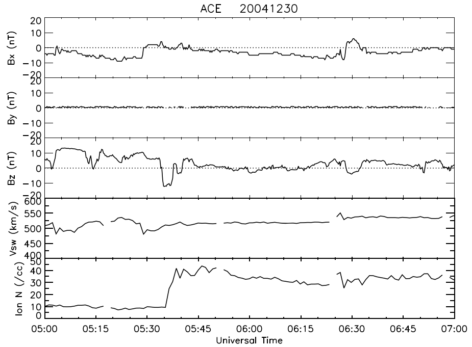
Figure 1. From the top to the bottom are plotted the interplanetary magnetic field, B_x , B_y and B_z and the solar wind velocity ( V_{sw} ) and density ( Ion\ N ) detected by ACE at L1 point for the SC event 1 on 30 December 2004. The SC was caused by the increase in N at 0535 UT.
