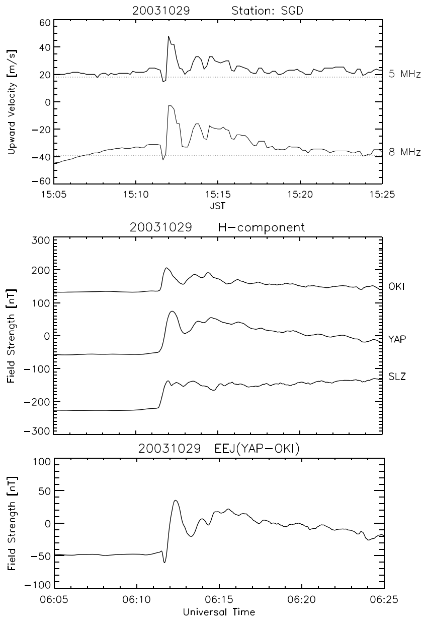
Figure 6. (top) Vertical motion of the ionosphere as observed with the HF Doppler sounder, (middle) H component magnetic fields at OKI, YAP, and SLZ, and the EEJ for (bottom) the SC event 4 on 29 October 2003. The ionosphere moves downward at the beginning of the MI while it moves upward during the whole period of the MI and is well correlated with the EEJ. The initial downward motion is well correlated with the negative EEJ of the PI of SC.
