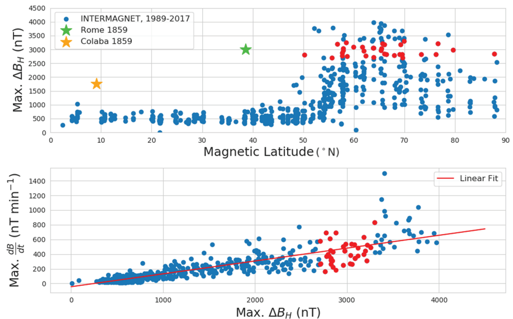
Figure 5. (top) Maximum \Delta B_H versus magnetic latitude for the 10 largest geomagnetic storms since 1989. The maximum Rome and Colaba \Delta B_H for 1859 are shown as green and orange stars, respectively. (bottom) Maximum \text{dB}/\text{dt}_{\min} versus \Delta B_H for the 10 largest geomagnetic storms since 1989. A \Delta B_H value of 3,000 nT corresponds to a maximum \text{dB}/\text{dt} of 477 \text{nT min}^{-1} . In both plots, the red dots indicate the stations with \Delta B_H between 2,700 and 3,300 nT.
