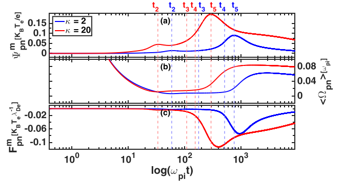
FIG. 7. The evolution of the (a) maximum ponderomotive potential ( \Psi_{pn}^m ), (b) average ponderomotive frequency ( \langle \Omega_{pn} \rangle ), and (c) the maximum ponderomotive force ( F_{pn}^m ) for Run-1(Vc) and Run-8(Vc).
