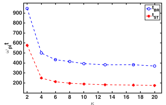
FIG. 10. Breaking and steepening time of the long-wavelength IASW as a function of the superthermal index. For this profile, we consider the fixed perturbation form with l_0 = 30 and \Delta n = 0.4 in all simulation runs.
