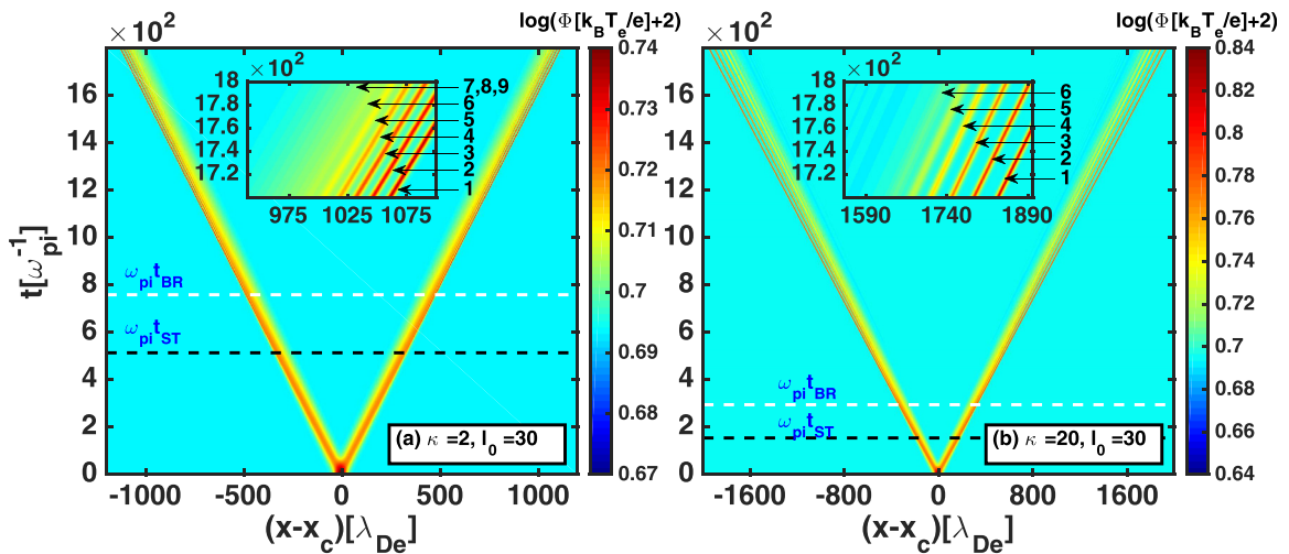
FIG. 3. The spatial and temporal evolution of the electrostatic potential in the system for the case Run-1(Vc) ( l_0 = 30 , \Delta n = 0.4 , \kappa = 2 ), and Run-8(Vc) ( l_0 = 30 , \Delta n = 0.4 , \kappa = 20 ). The inset shows the zoomed portion of the right side propagating pulses. In this, the dark red and yellow bands correspond to the IASW pulses, whereas the alternate dark and light blue bands are due to the IA oscillations. The black and white horizontal dashed lines indicate the steepening ( \omega_{pi}t_{ST} ) and breaking ( \omega_{pi}t_{BR} ) time of the wave, respectively. The numbers represent the IASW pulse number in the chain. It may be noted that in panel-(a), the pulses 7, 8, and 9 are not yet evolved to form distinct solitary pulses. Hence, they are shown by just a single arrow. At the final stage, 9 and 6 number of solitons are formed in Run-1(Vc) and Run-8(Vc), respectively.
