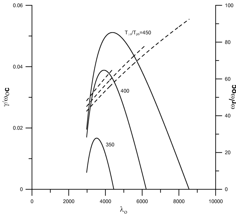
FIG. 5. Variation of normalized real frequency \omega_r/\omega_{oc} (---) and growth rate \gamma/\omega_{oc} (—) vs normalized wave number ( \lambda_o ) for J=1 , and T_{\perp o}/T_{pb} = 350, 400, 450 , respectively, shown as curves 1, 2, and 3. The other parameters are the same as in Fig. 1.
