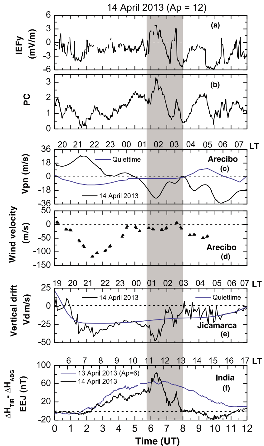
Figure 2. Variation in (a) propagation time lag corrected IEFy (in mV/m), (b) polar cap (PC) index, (c) averaged perpendicular north plasma drift (Vpn in m/s) over Arecibo along with seasonal quiet time variations (in blue line) from Fejer (1993), (d) variations of meridional wind velocity over Arecibo where the positive value indicates poleward and negative for equatorward, (e) ISR measured vertical plasma drift over Jicamarca (Vd in m/s) in black along with quiet time vertical drift (in blue line) from Scherliess and Fejer (1999) where the vertical drift is positive upward, and (f) equatorial electrojet strength (EEJ in nT) over India in black, which is overlaid with a quiet day (14 April 2013) EEJ variation in blue during 0000–1200 UT. The gray shaded region (0545–0800 UT) marks the interval when PP/OS electric field perturbations are seen over Arecibo/Jicamarca and Indian sector. IEF = interplanetary electric field.
