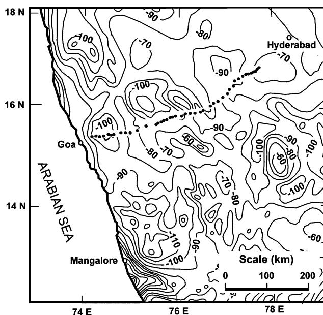
Figure 2. Bouguer gravity map of the granite–greenstone belt in the South Indian Shield. The MT stations are marked by solid circles.
